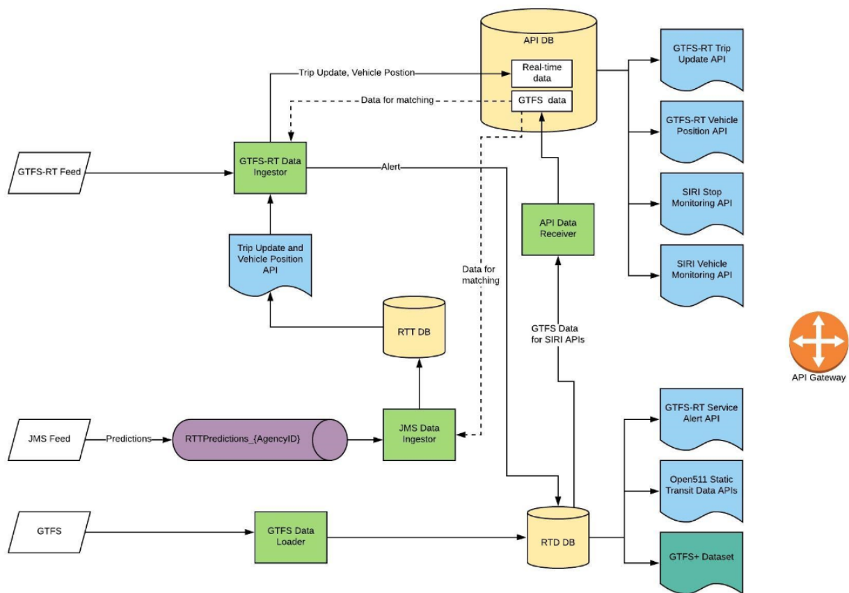
Figure 1 – Transit data communication architecture for San Francisco Bay Area 511
